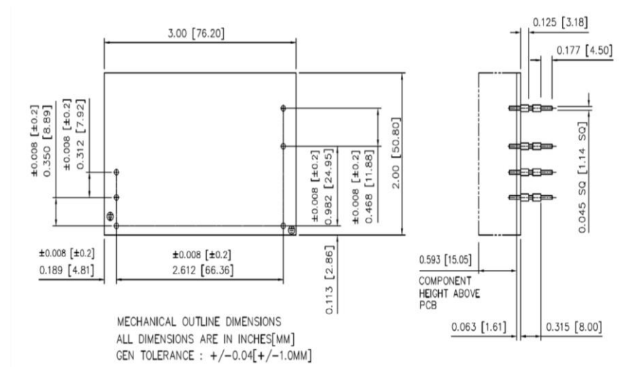
Mechanical Drawing – PCB Mount Option
